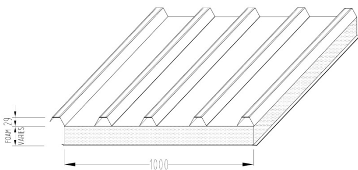
NORFOAM INSULATED PANEL (NORDECK)
